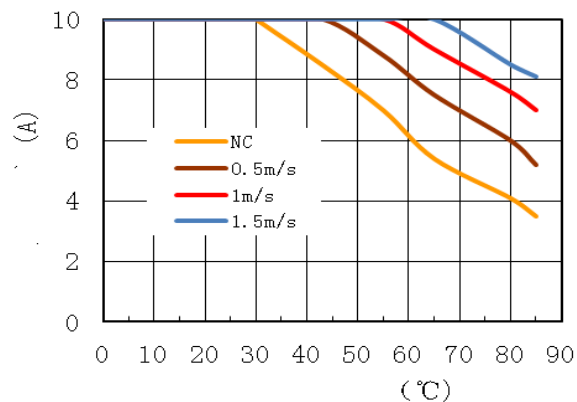
Derating (Vin=12Vdc)
