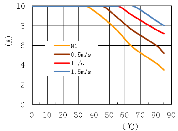
Derating (Vin=12Vdc)
