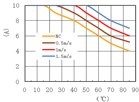
Derating (Vin=12Vdc)
