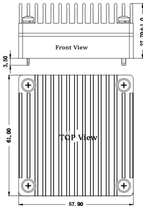
Standard+Heatsink 61*57.9*27.7mm
