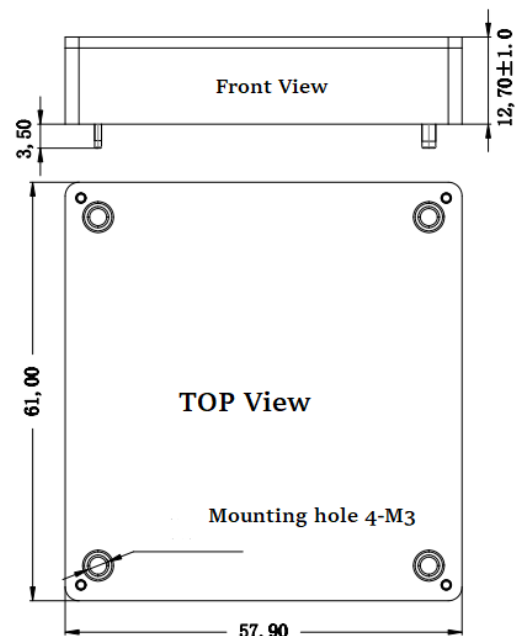
Standard 61*57.9*12.7mm
