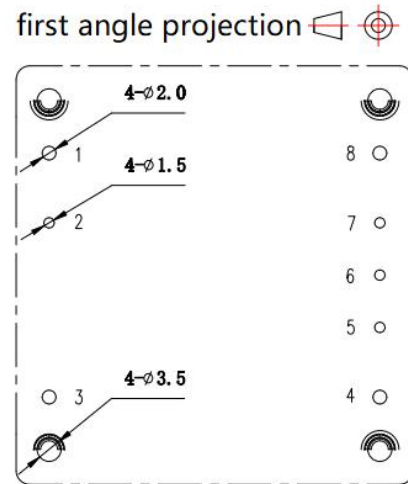
Recommended PCB Slot Size
