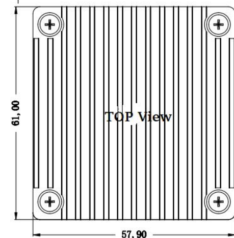
Standard+Heatsink 61*57.9*27.7mm
