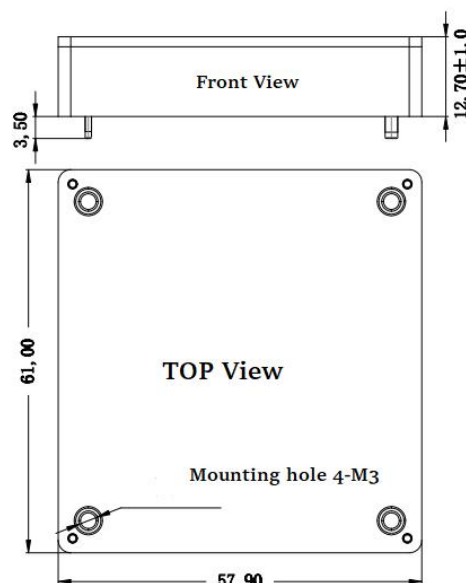
Standard 61*57.9*12.7mm
