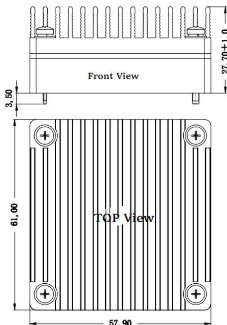
Standard+Heatsink 61*57.9*27.7mm
