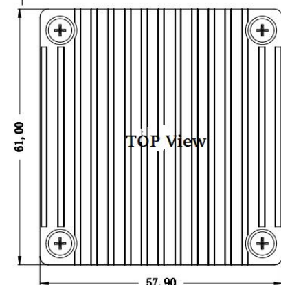
Standard+Heatsink 61*57.9*27.7mm
