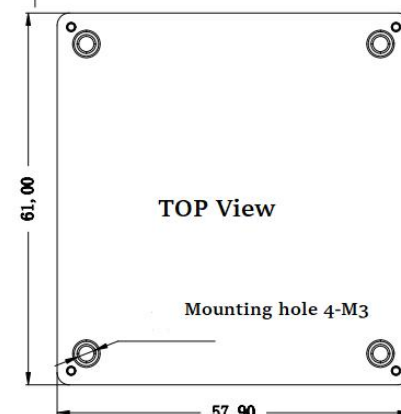
Standard 61*57.9*12.7mm
