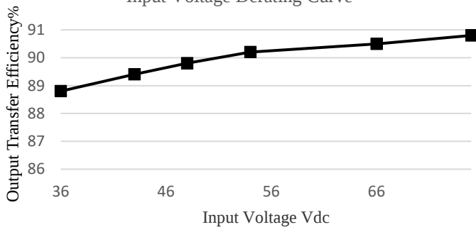
Input Voltage Derating Curve
