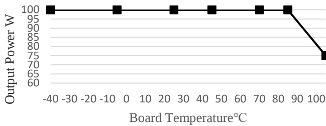
48V Input Derating Curve
