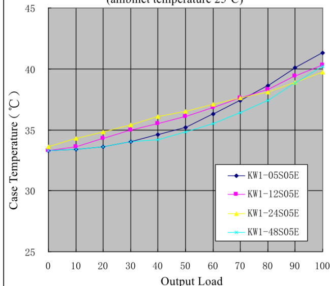
Case Temperature and Output Load Curve (ambient temperature 25°C)
