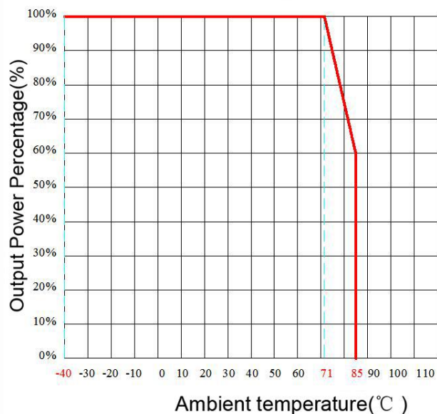
Temperature Derating Curve
