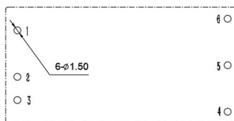
Recommended PCB holes size
