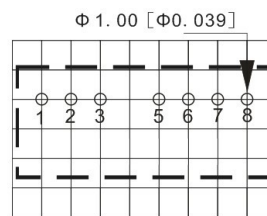
PCB layout vertical view Grid 2.54x2.54[0.10x0.10]
