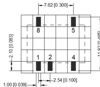
PCB layout vertical view (Grid 2.54x2.54mm)
