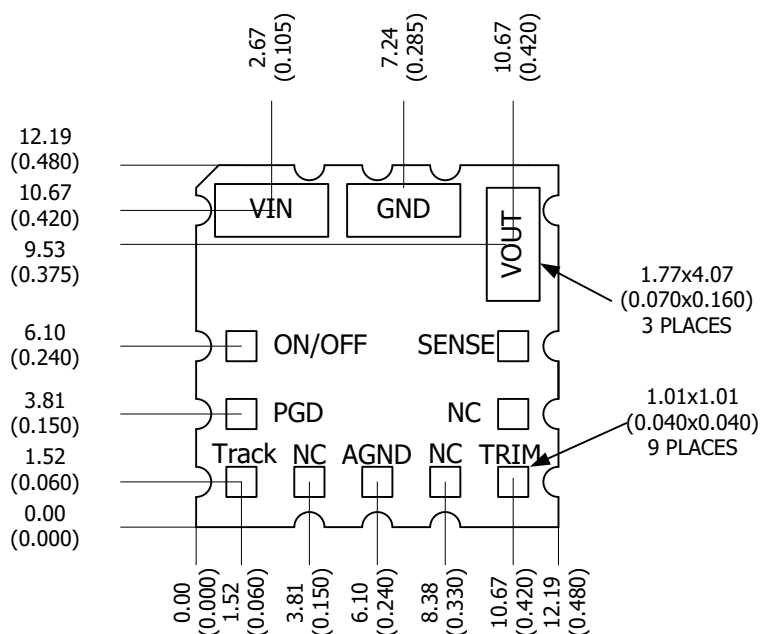
COMPONENT-SIDE FOOTPRINT
