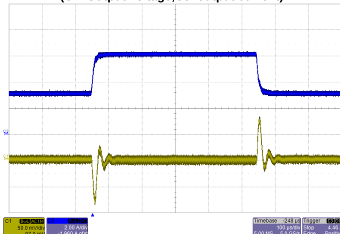
Transient Response V_{IN}=5V , Step from 3A~6A~3A (C2: Output,C3: Load current)
