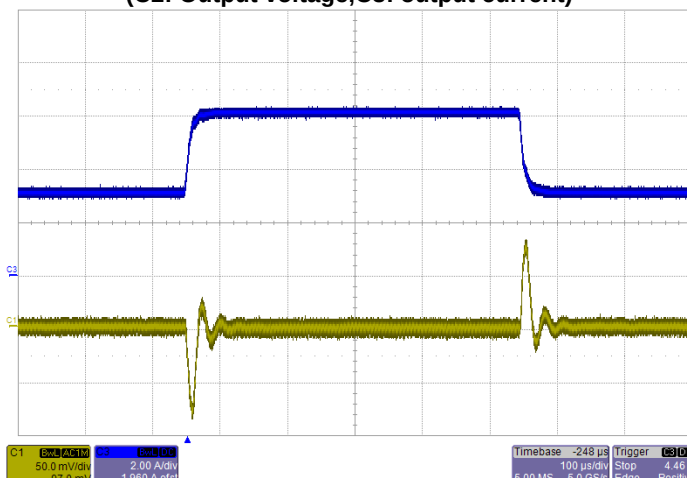
Transient Response V_{IN}=5V , Step from 3A~6A~3A (C1: Output,C3: Load current)
