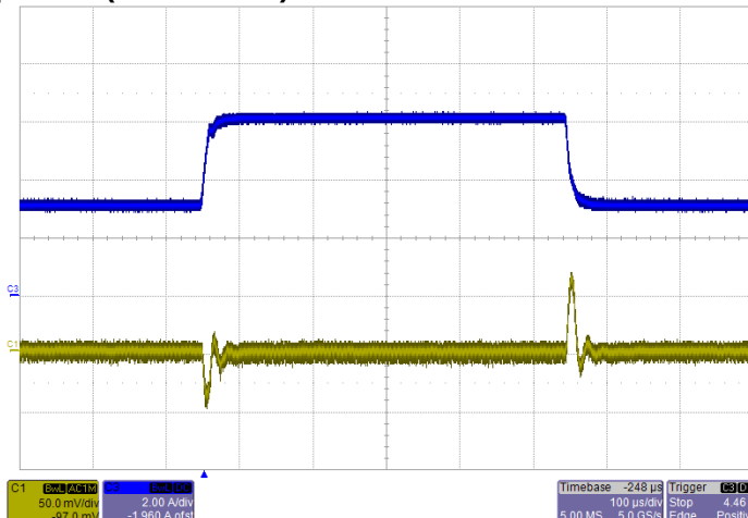
Transient Response V_{IN}=12V , Step from 3A~6A~3A (C2: Output,C3: Load current)
