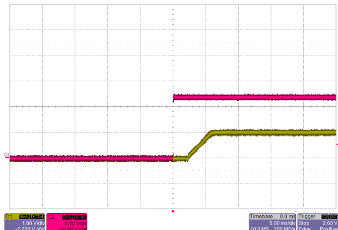
Start-up V_{IN}=12V , I_O=6A (C2: Output,C1: Input)
