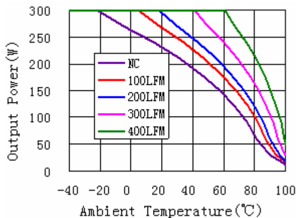
Derating curve with 0.95"HS radiator
