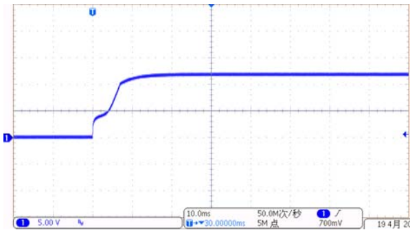
Rise Time
