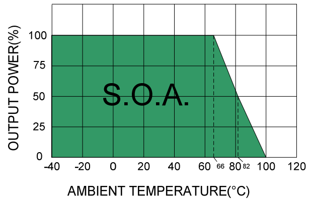
Derating Curve
