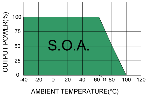
Derating Curve
